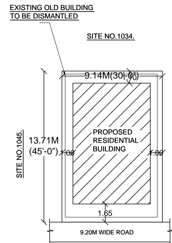
SITE PLAN
